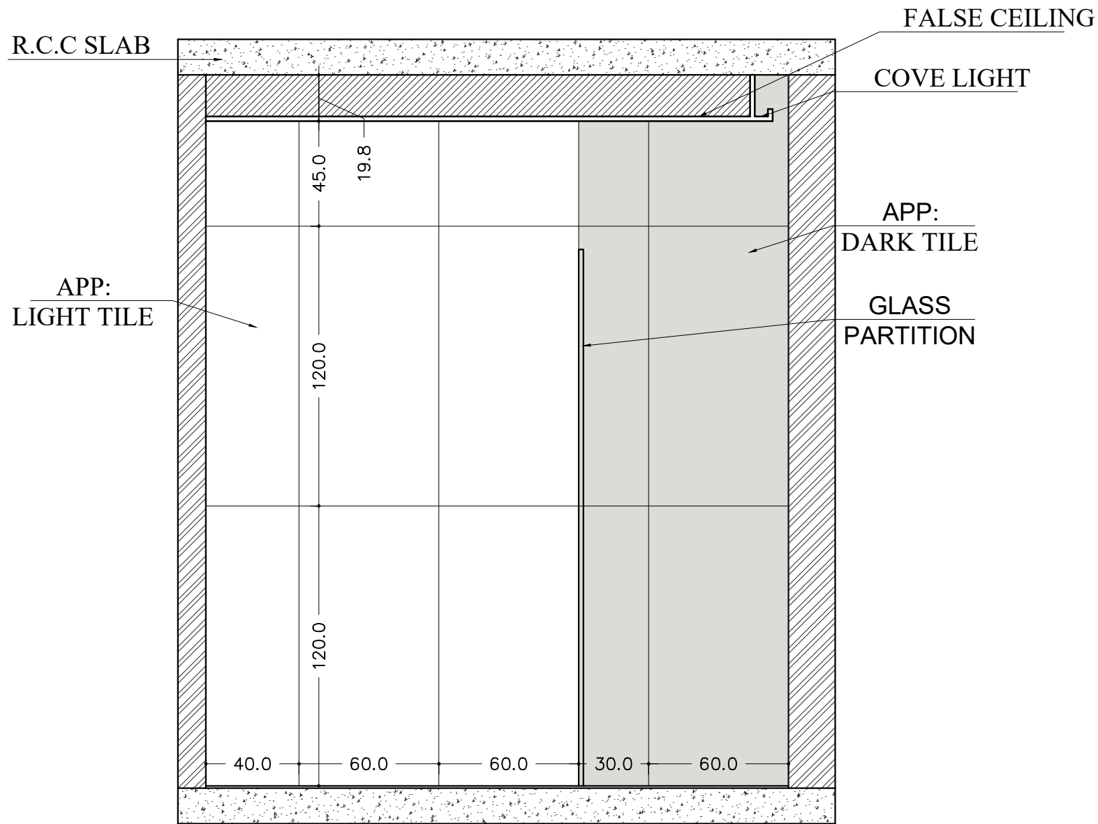
ELEVATION WORKING ELE-04
