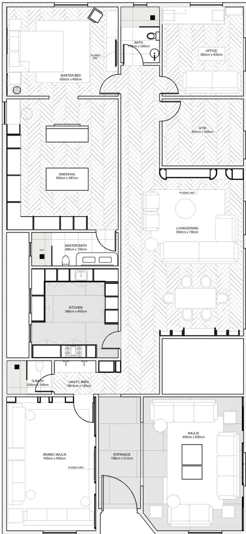
FURNITURE LAYOUT PLAN
