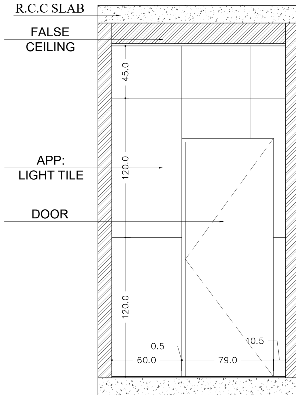
ELEVATION WORKING ELE—02
