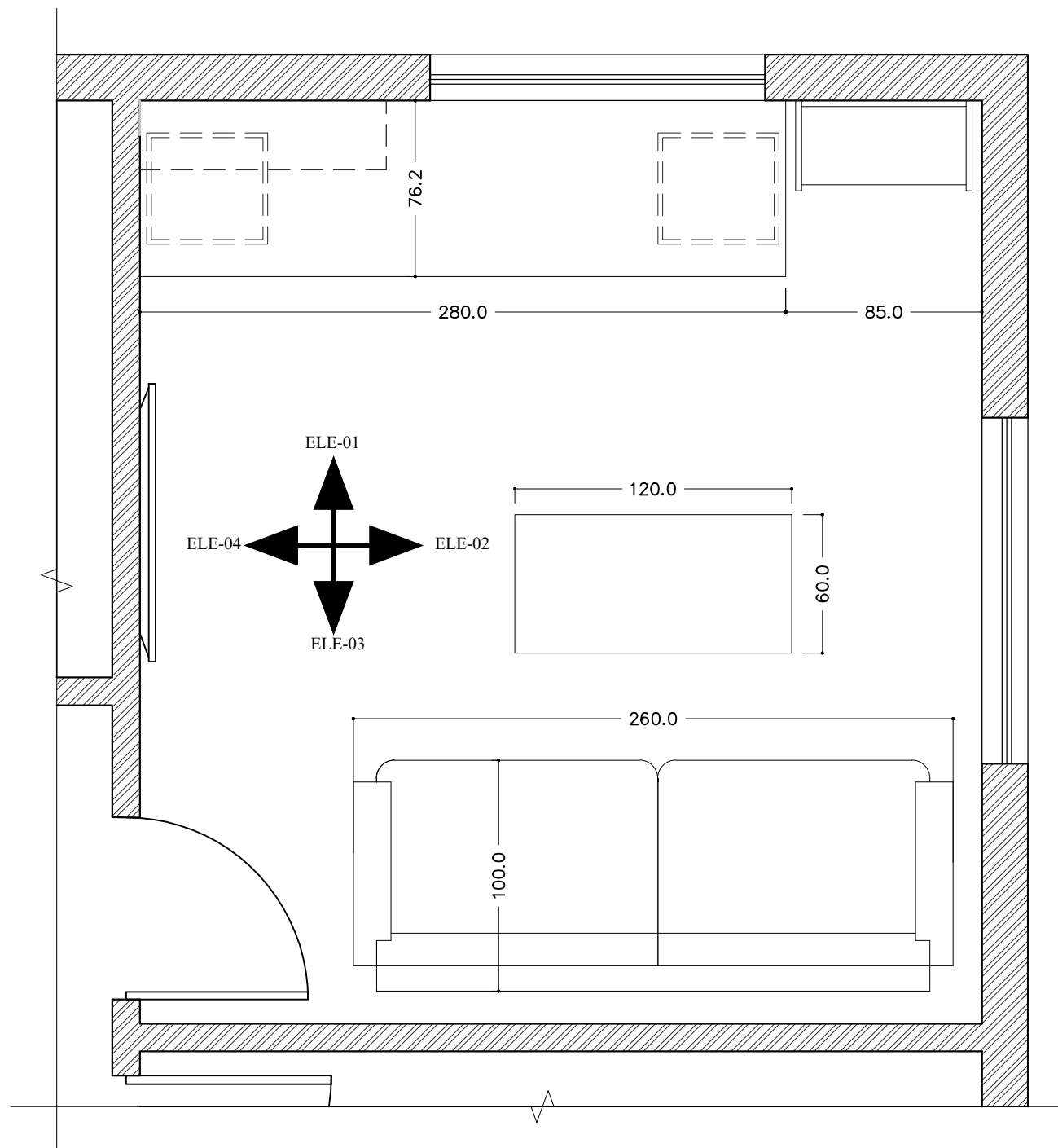
LAYOUT DIMENSION PLAN
