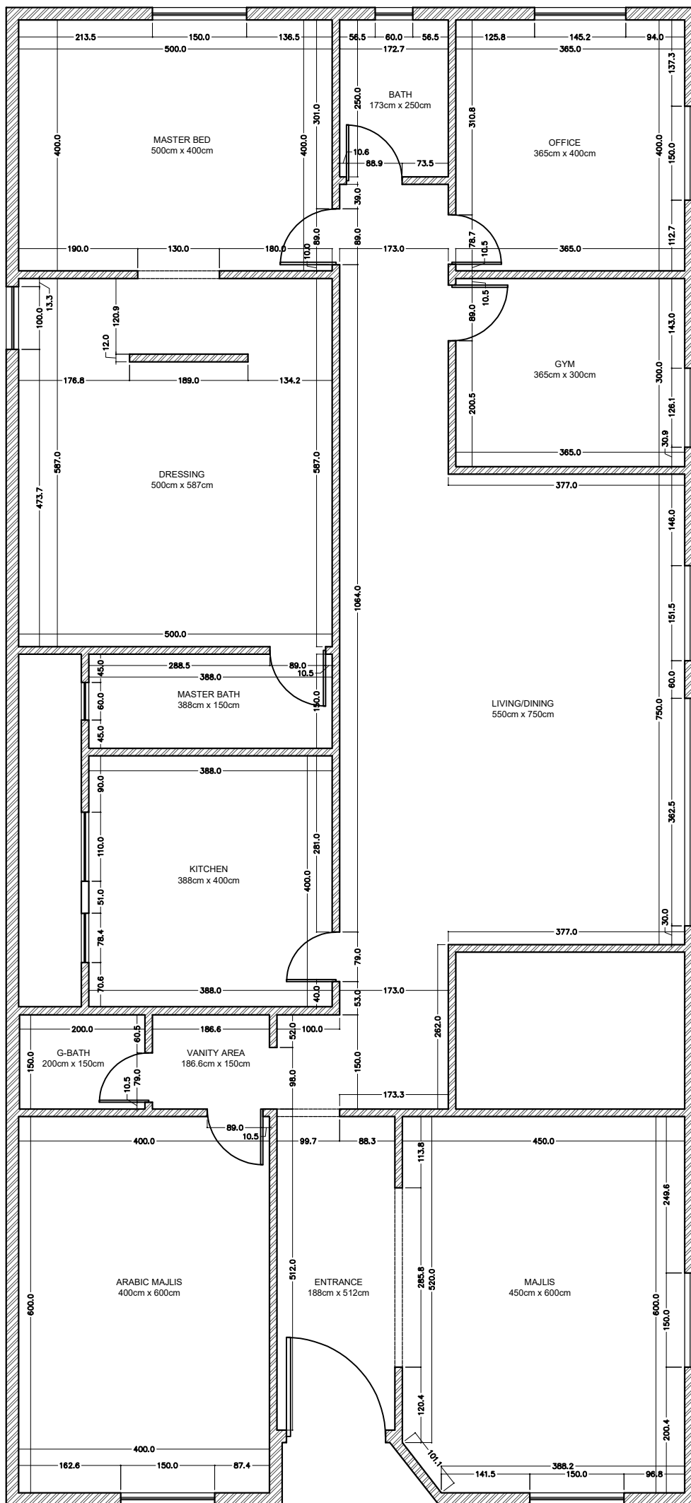
APARTMENT WORKING PLAN
