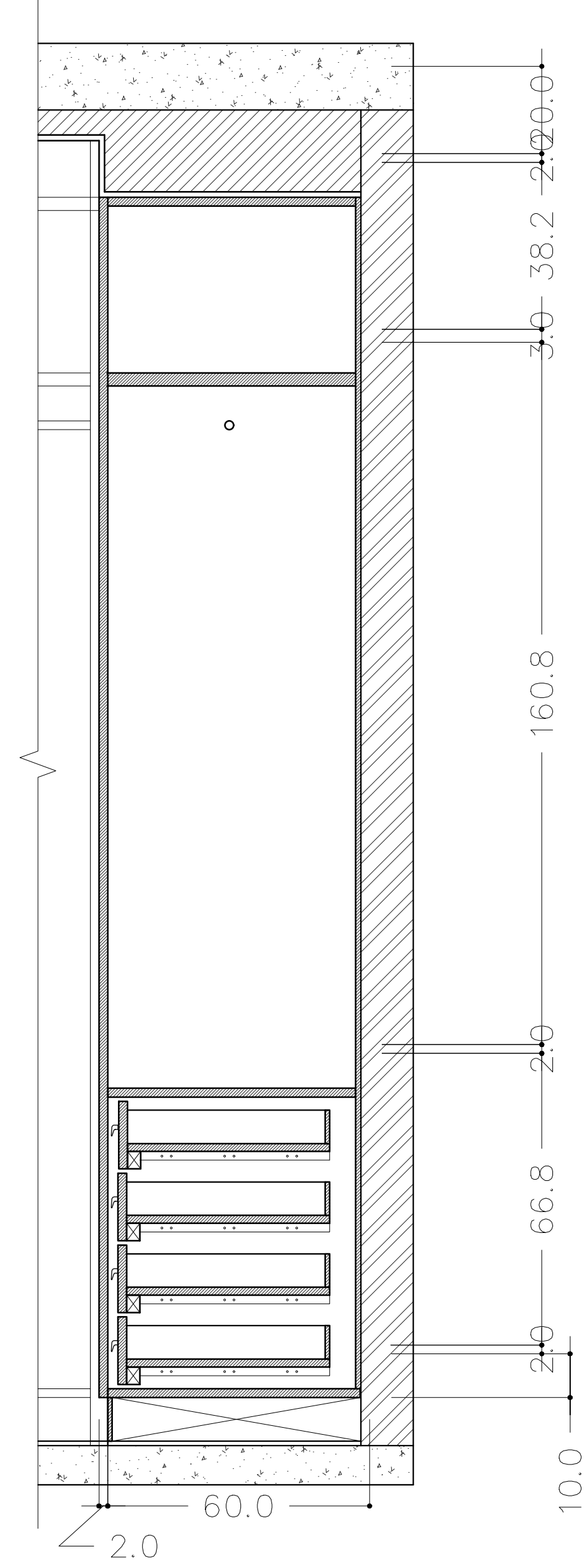
SECTION-03
