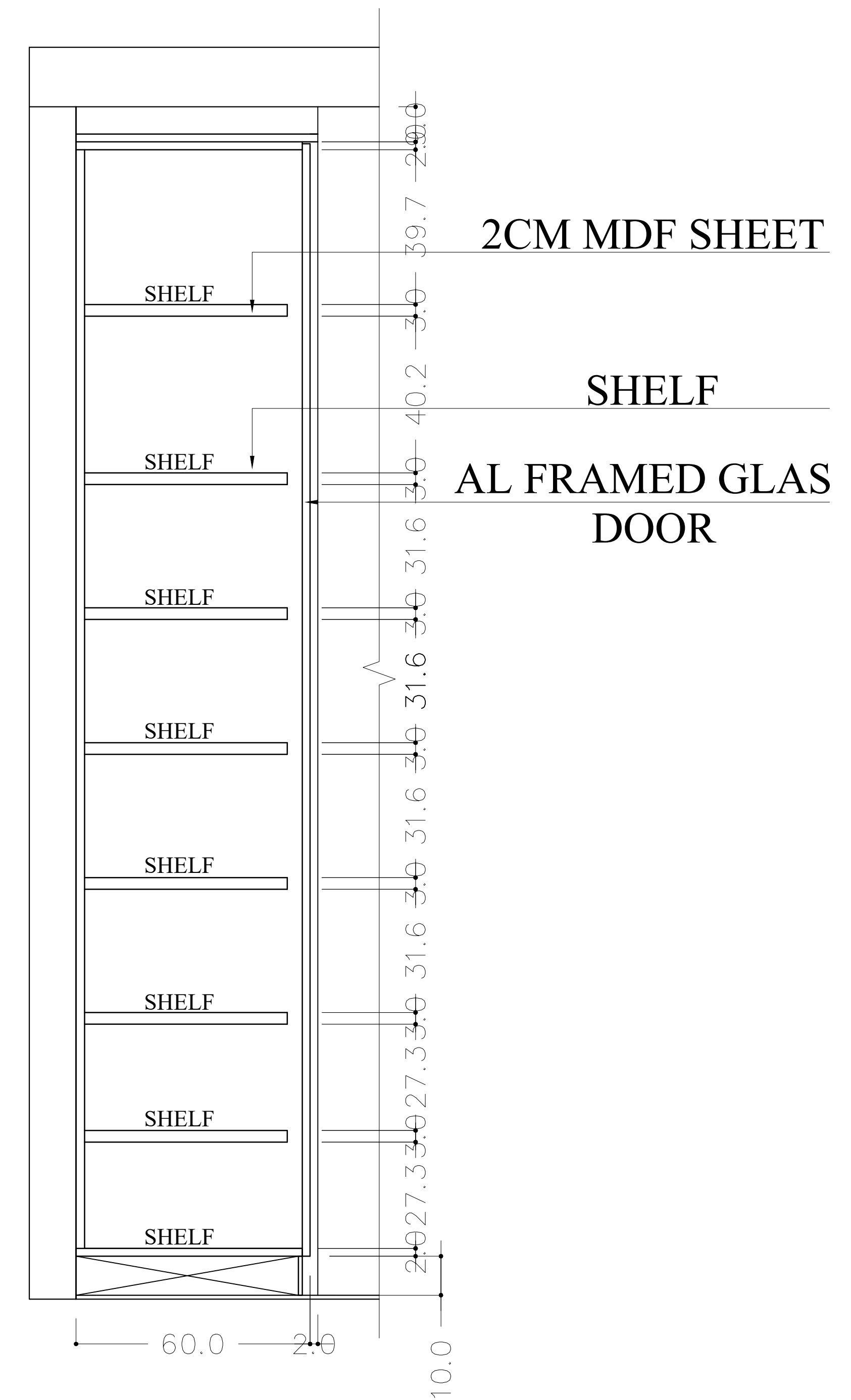
SECTION-02
