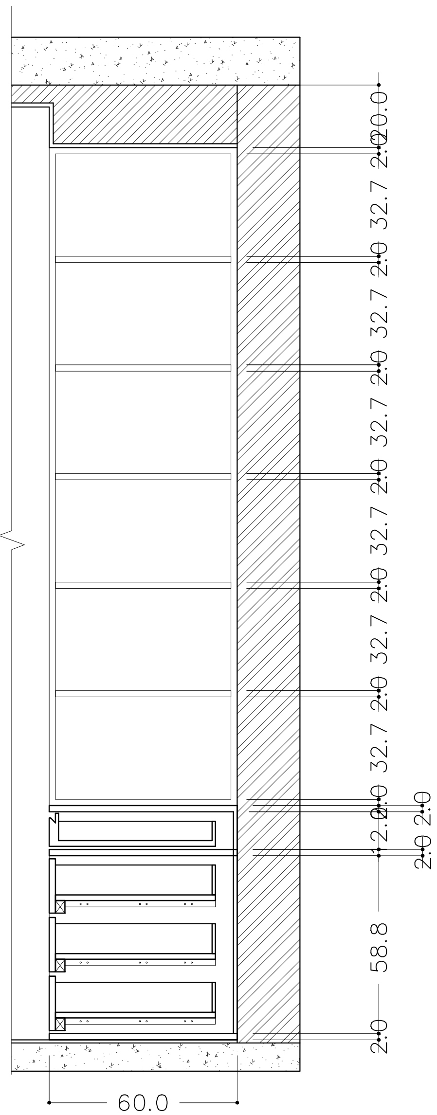
SECTION-02
