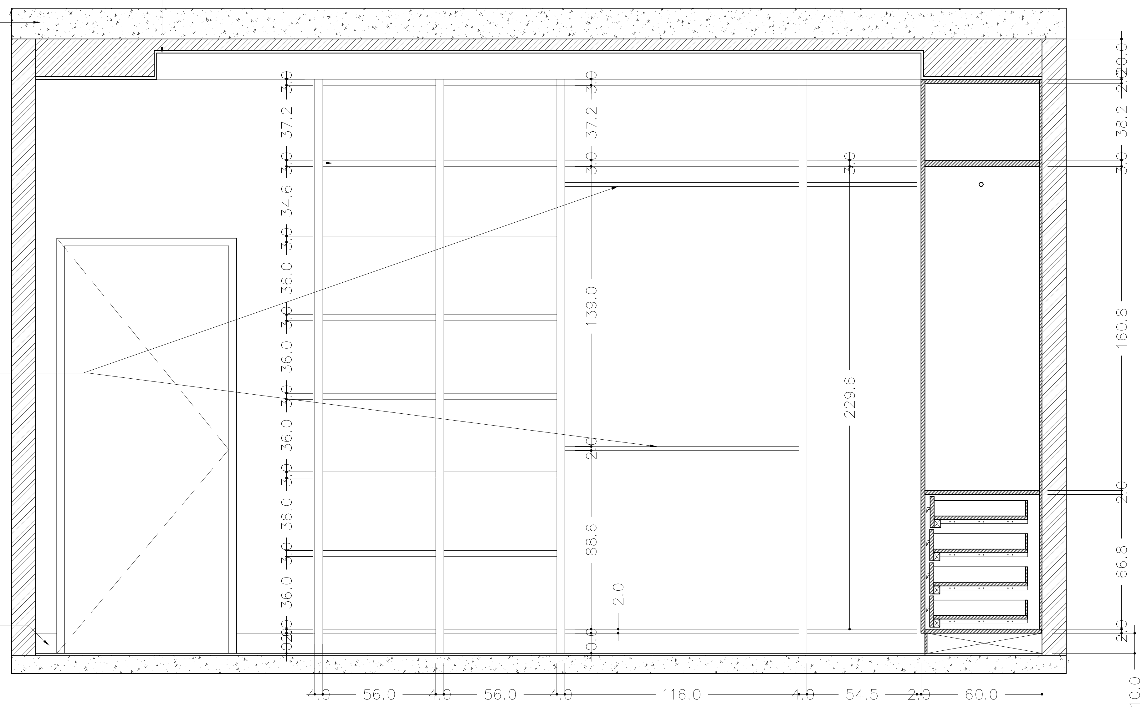
INNER PARTITION WORKING E-01
