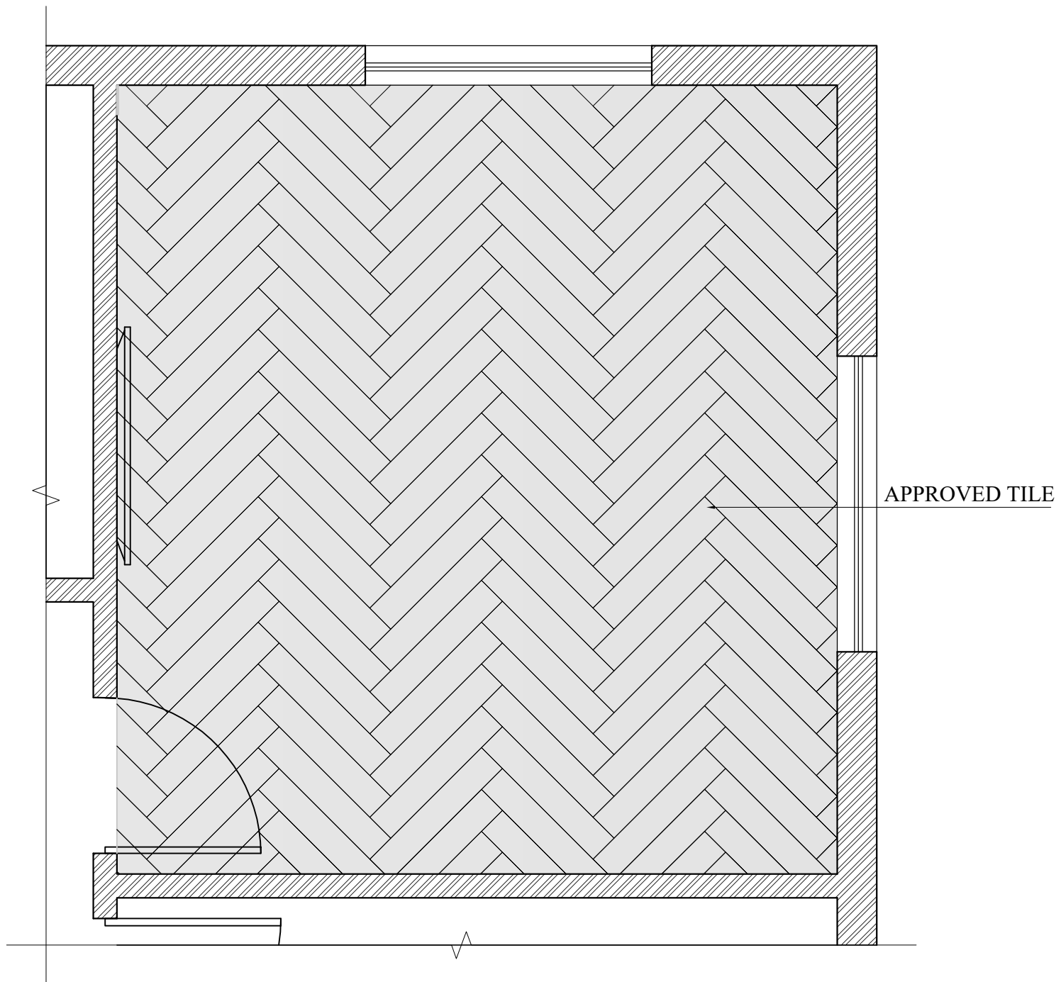
FLOORING LAYOUT PLAN
