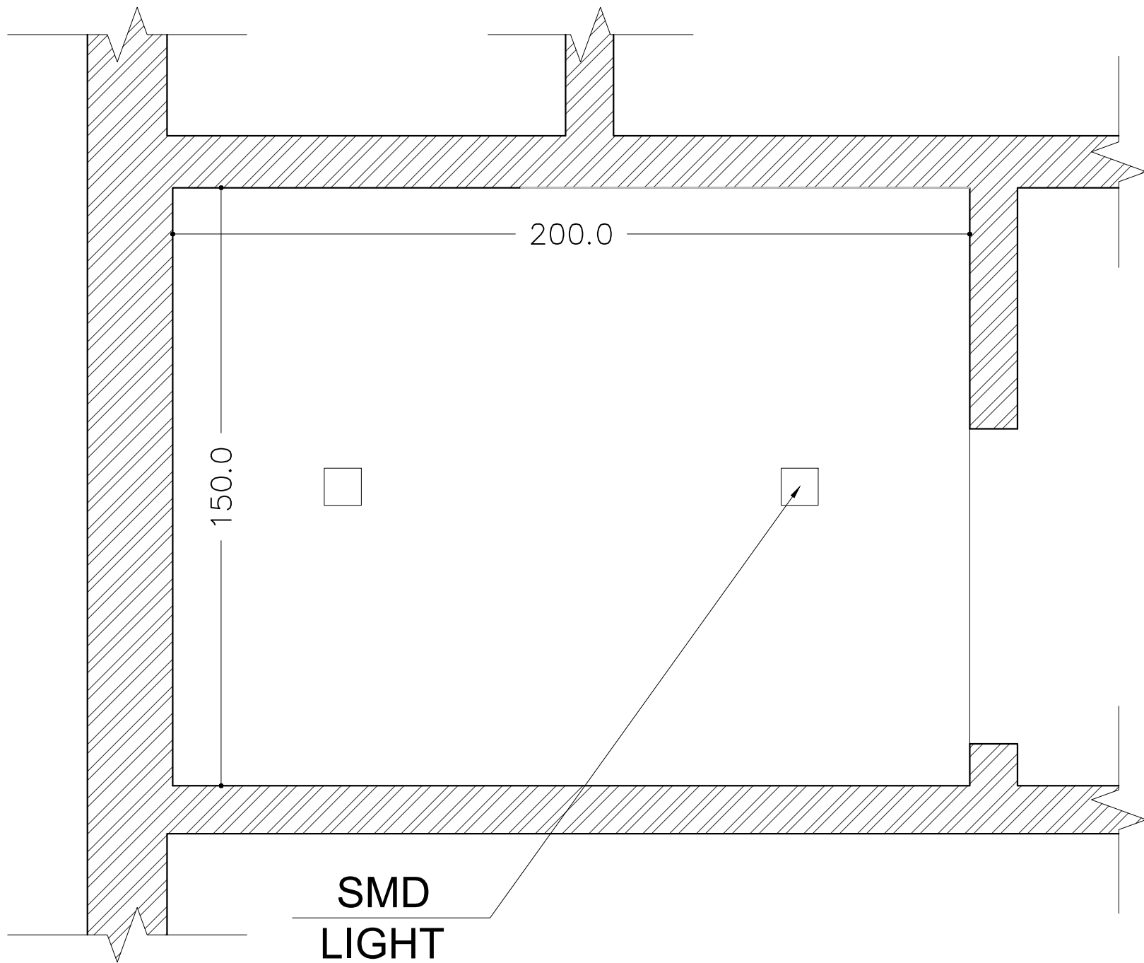
CEILING LAYOUT PLAN
