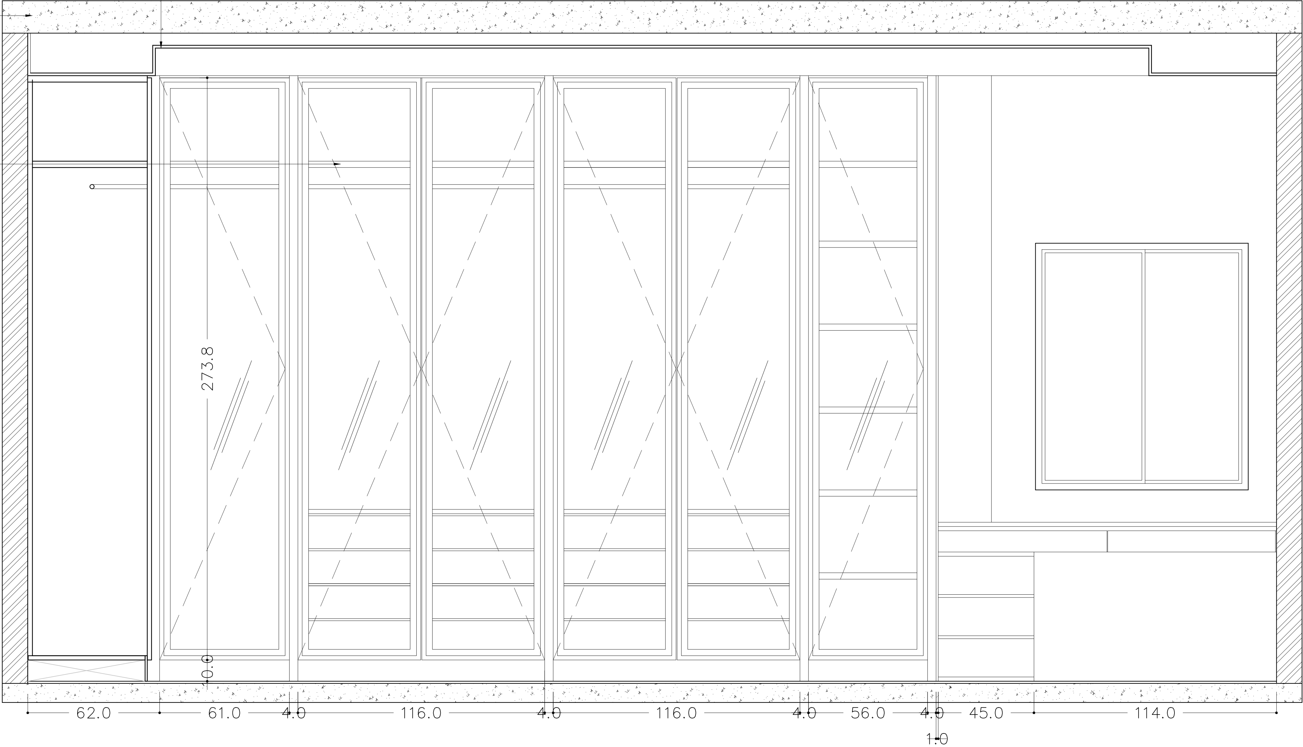
SHUTTER WORKING E-02
