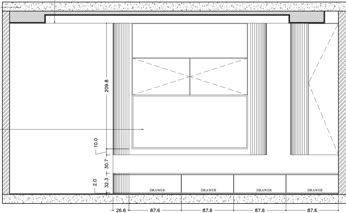
ELEVATION WORKING ELE-01
