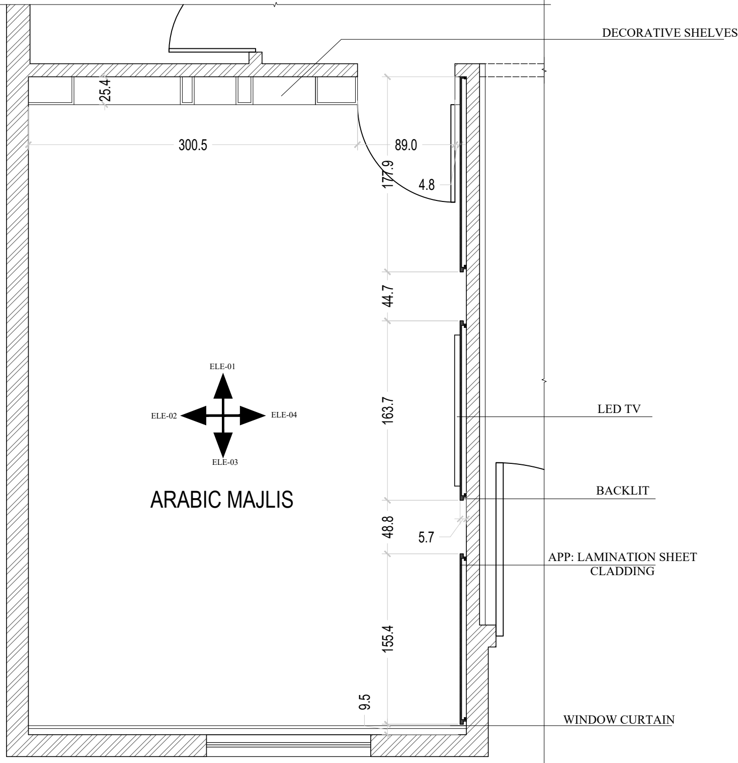
DIMENSIONS LAYOUT PLAN
