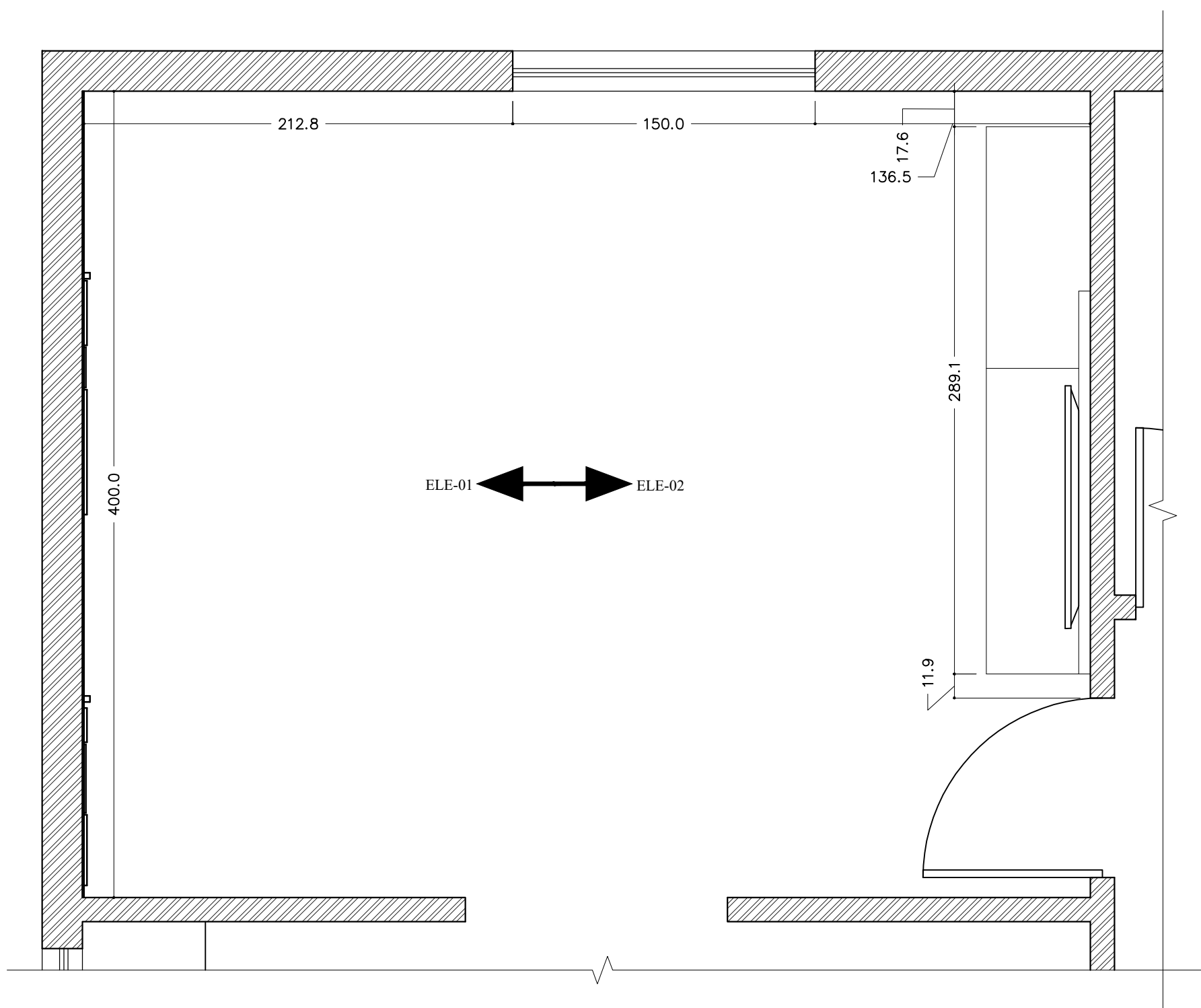
LAYOUT DIMENSION PLAN
