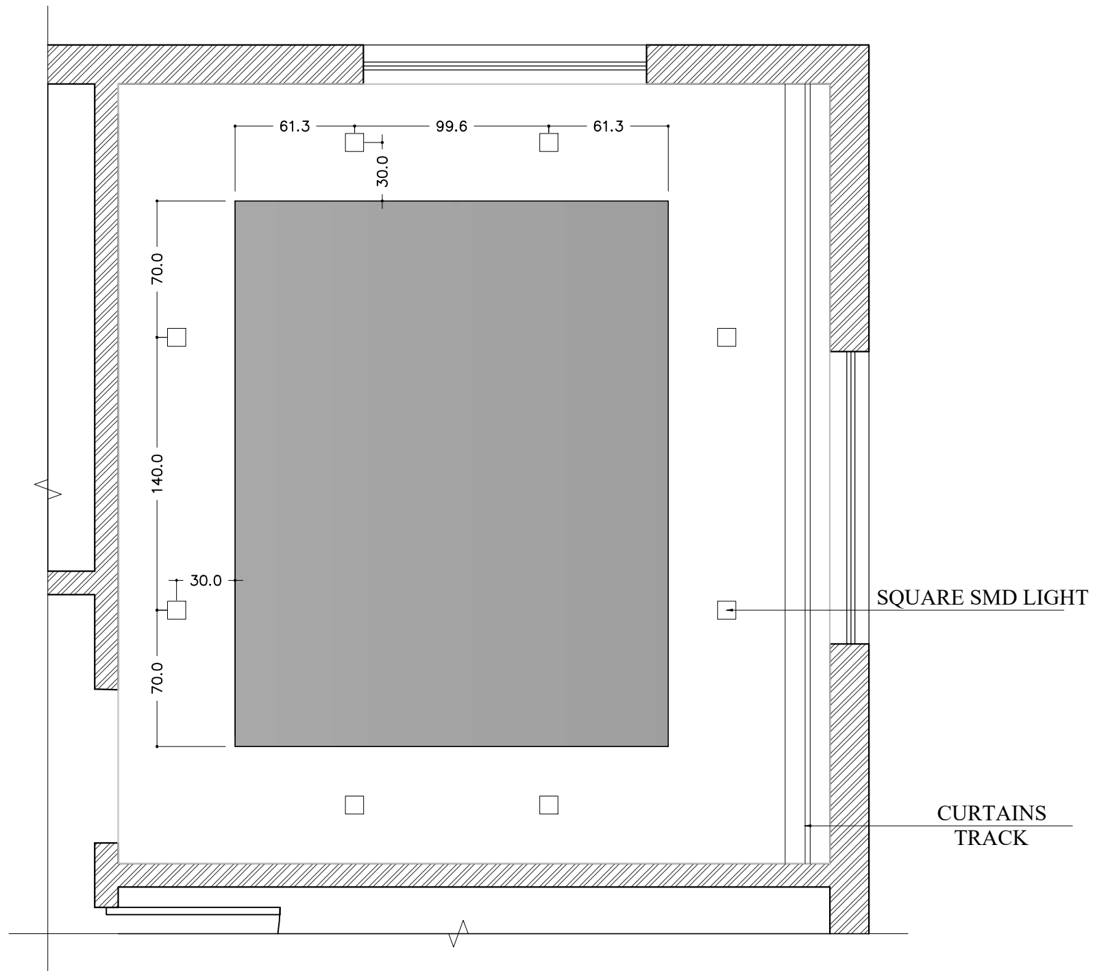
CEILING LIGHT POINT WORKING
