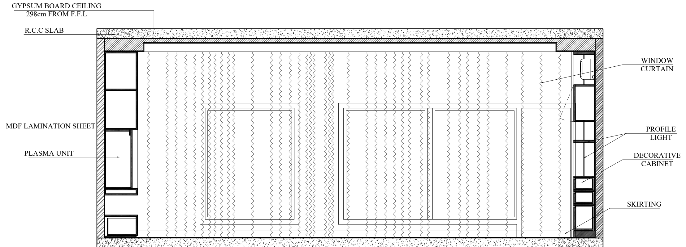
ELEVATION WORKING E-03
