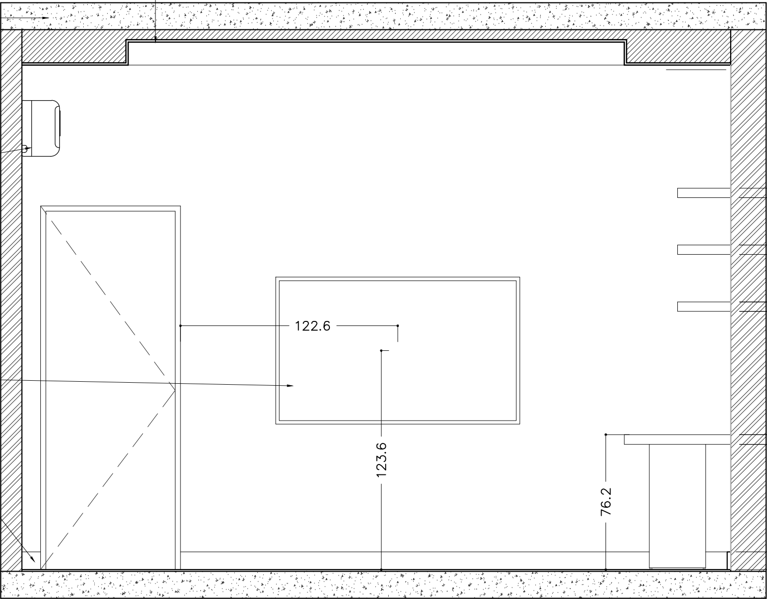
ELEVATION WORKING ELE-04
