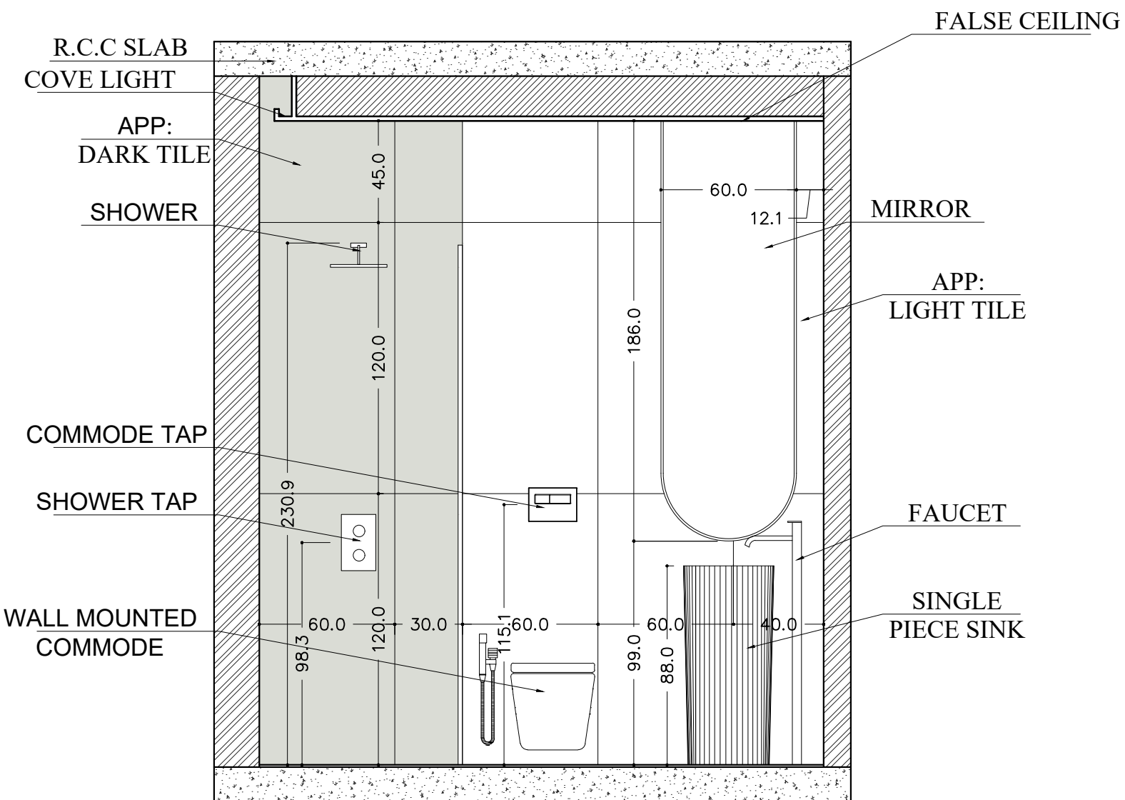
ELEVATION WORKING ELE-02
