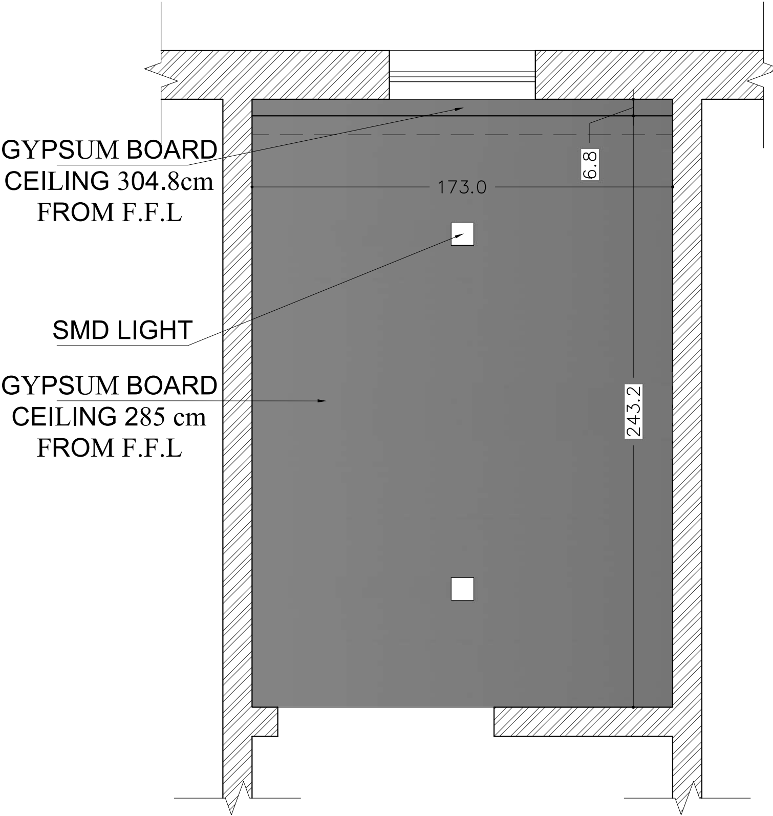
CEILING LAYOUT PLAN
