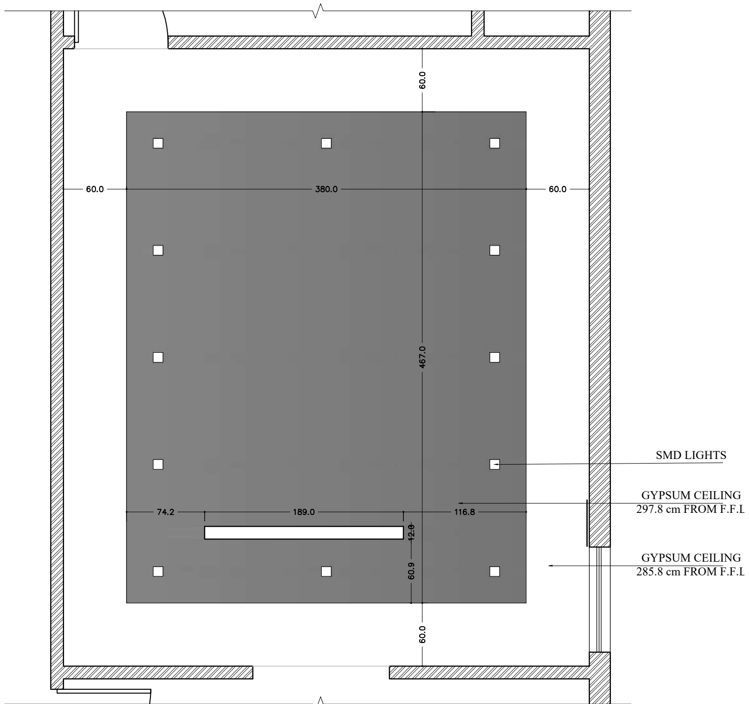
CEILING LAYOUT PLAN
