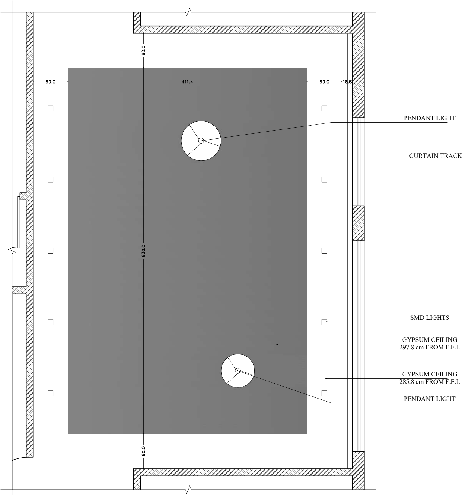
CEILING LAYOUT PLAN
