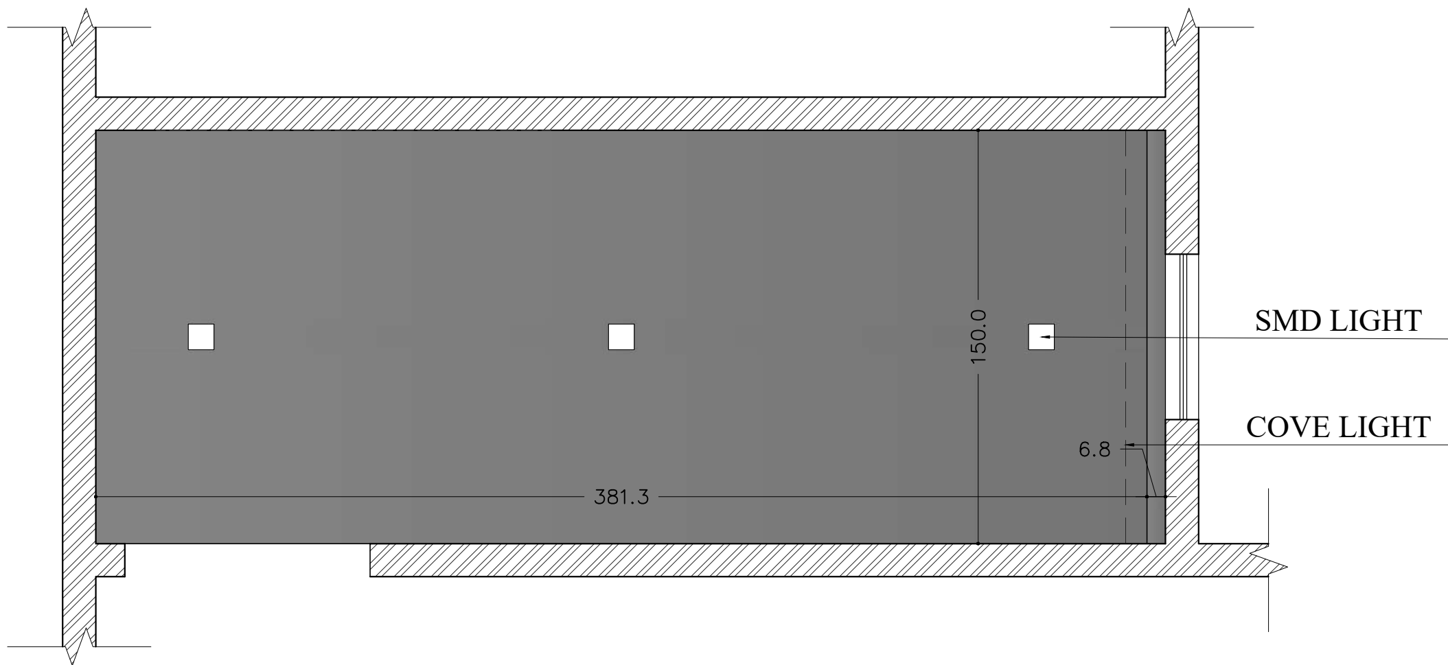
CEILING LAYOUT PLAN
