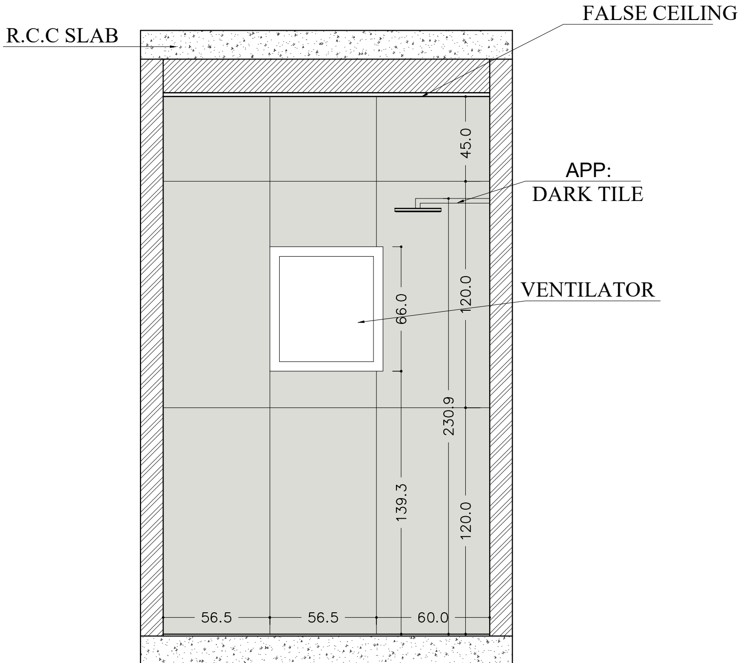
ELEVATION WORKING ELE—01
