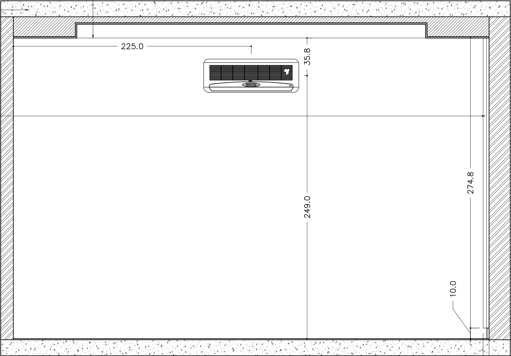
ELEVATION WORKING ELE-01
