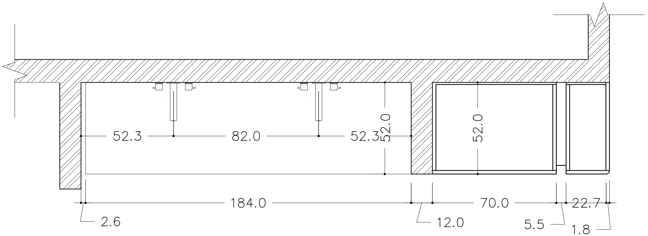
VANITY AREA PLAN
