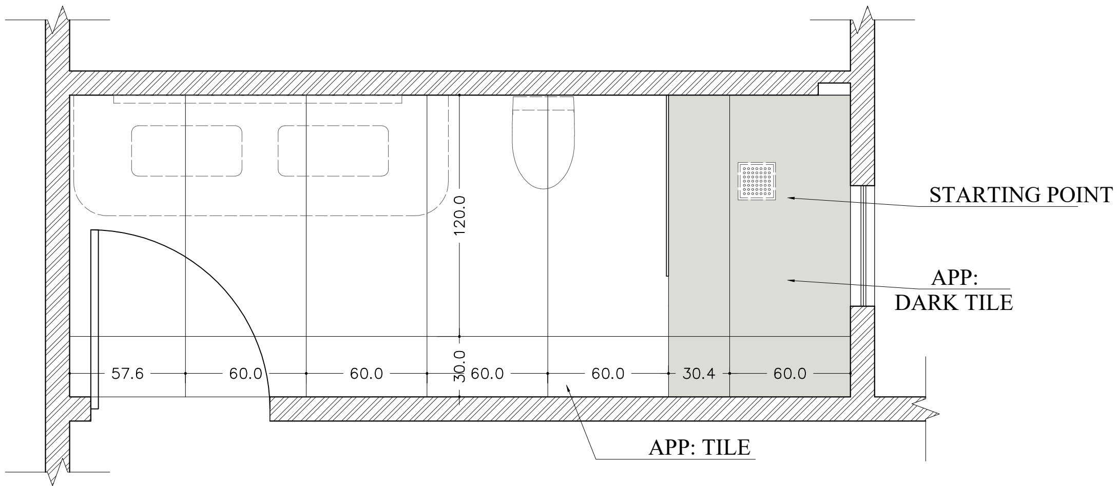
FLOORING LAYOUT PLAN
