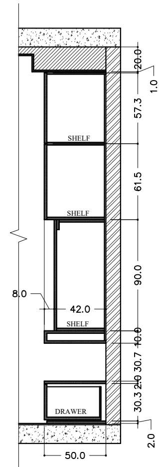
SECTION-01
