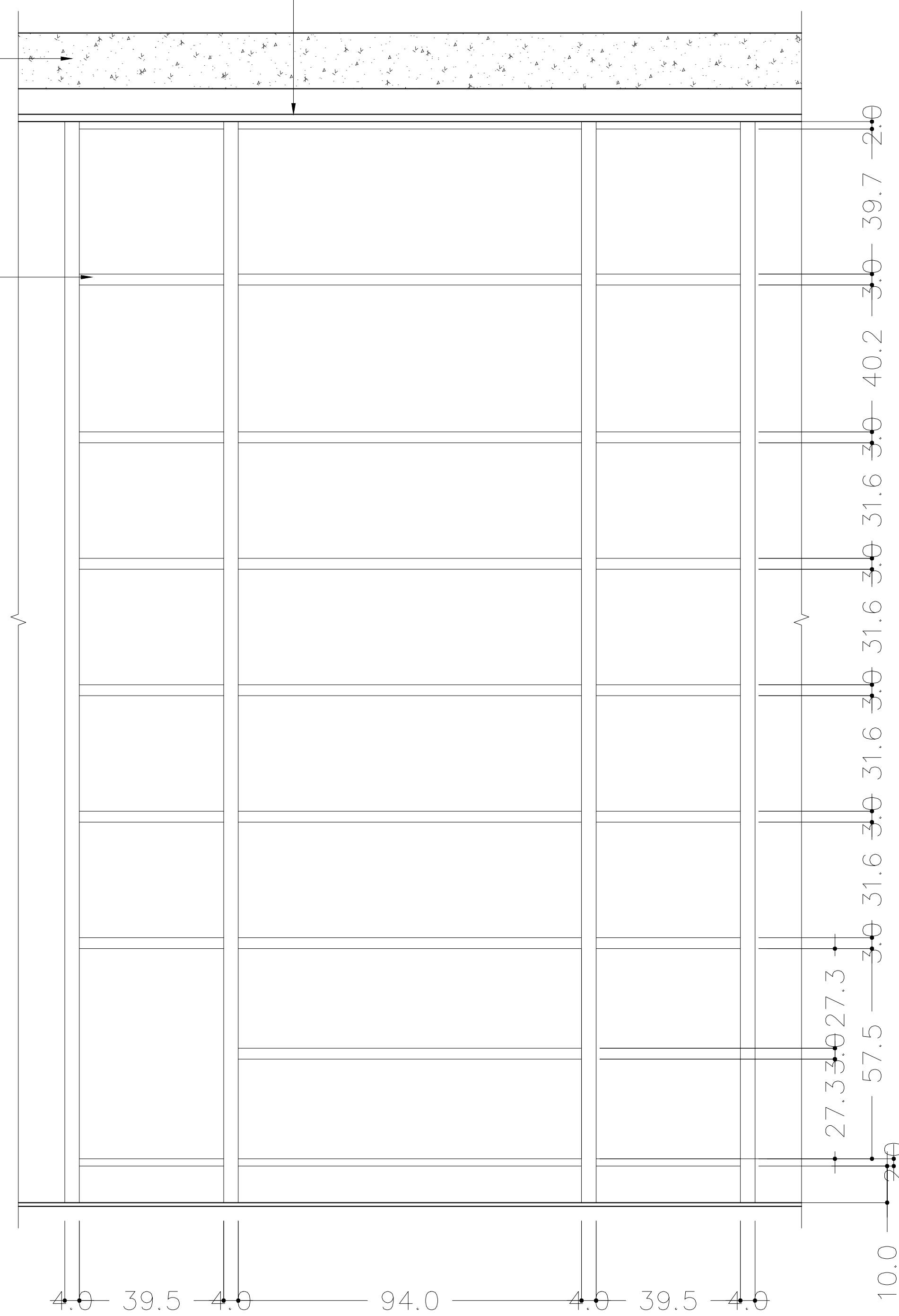
INNER PARTITION WORKING-03
