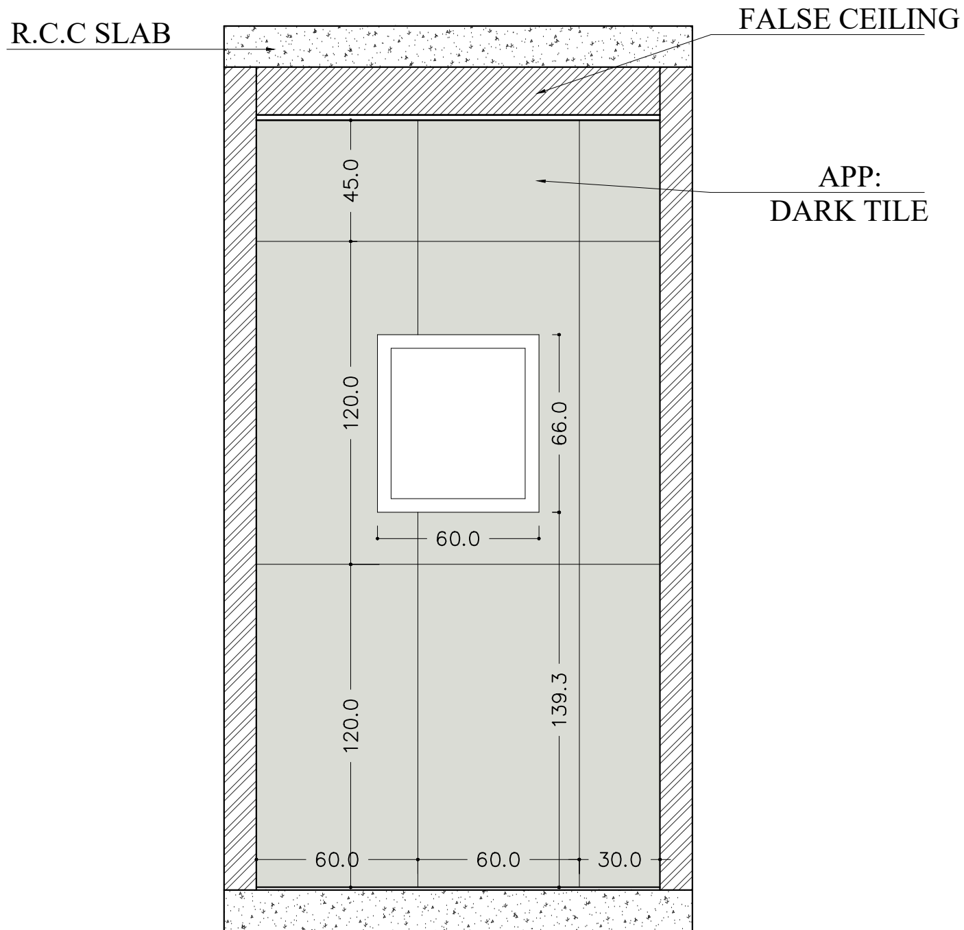
ELEVATION-02
