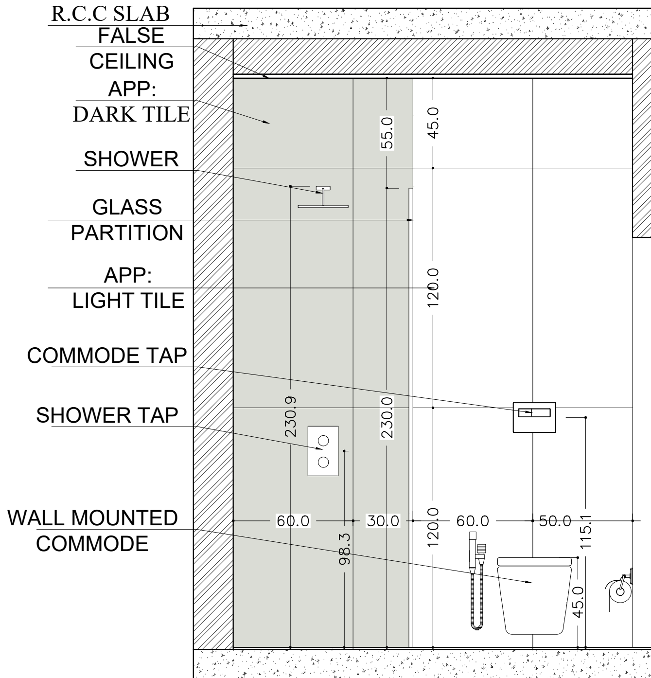
ELEVATION WORKING ELE-01
