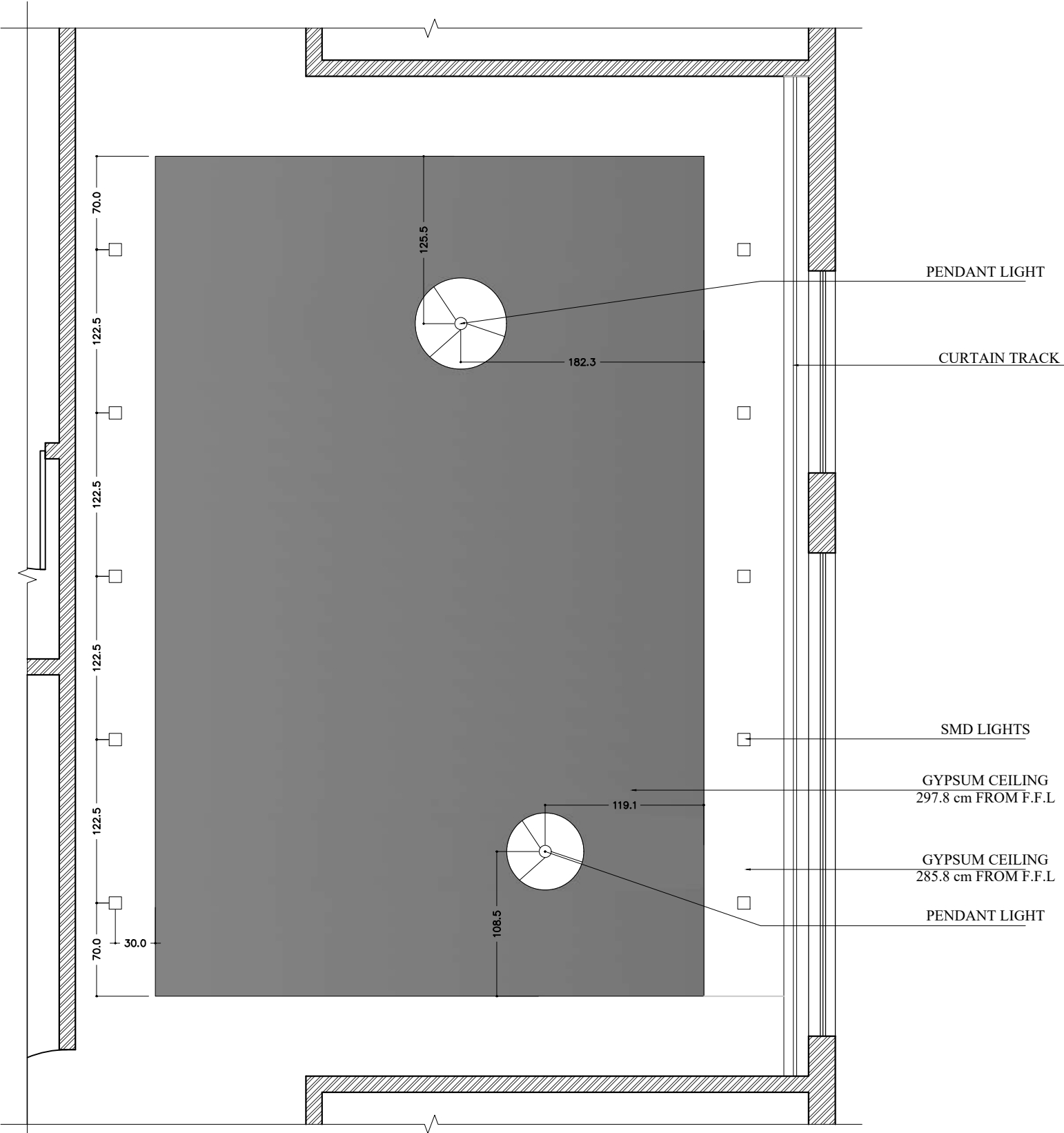
CEILING LIGHT POINT WORKING
