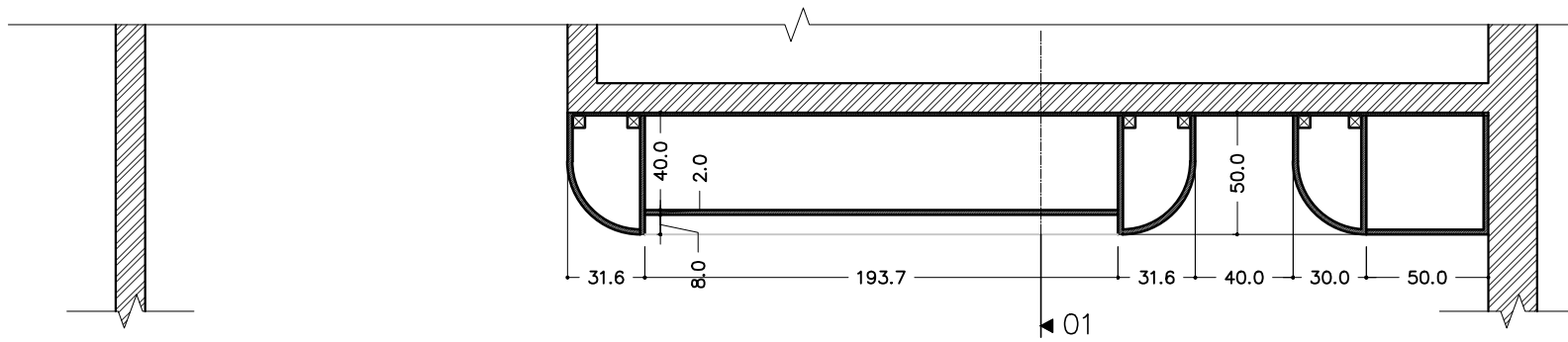
WORKING PLAN E-01
