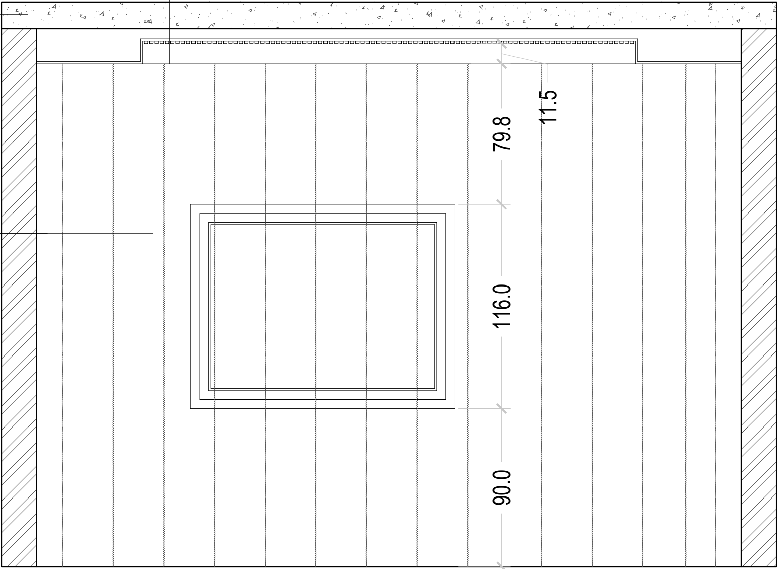
ELEVATION 03
