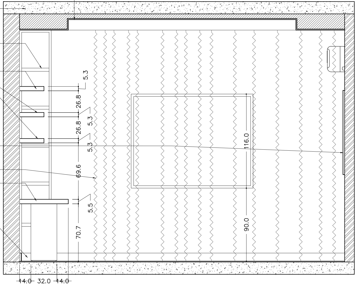
ELEVATION WORKING ELE-02
