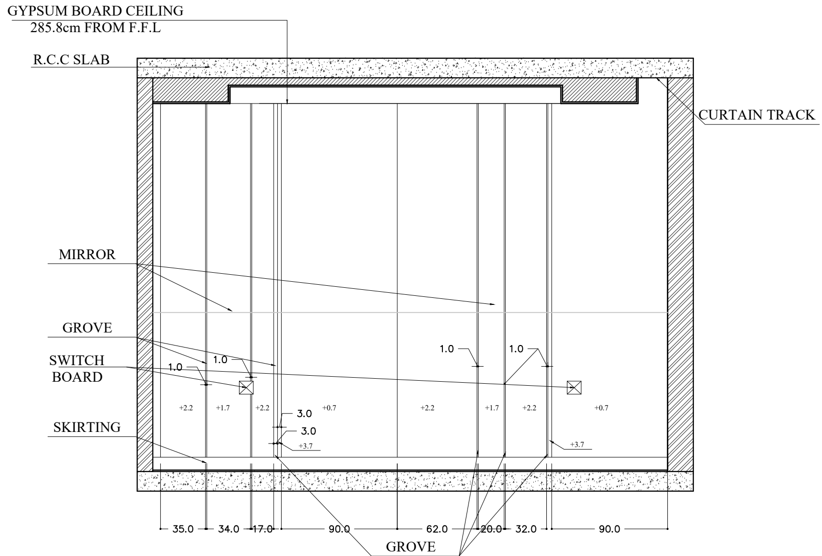
WORKING ELEVATION E-01
