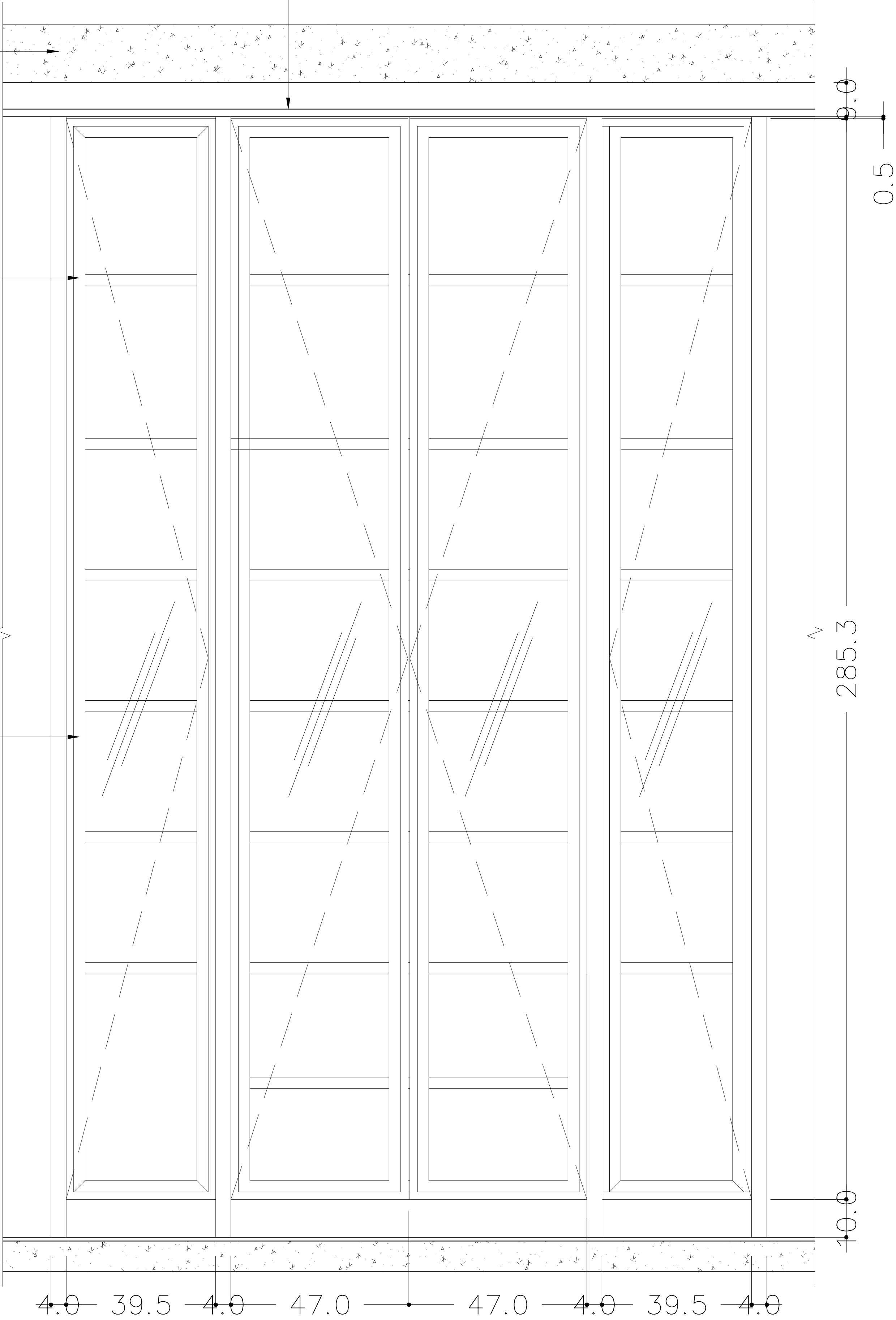
SHUTTER WORKING E-03
