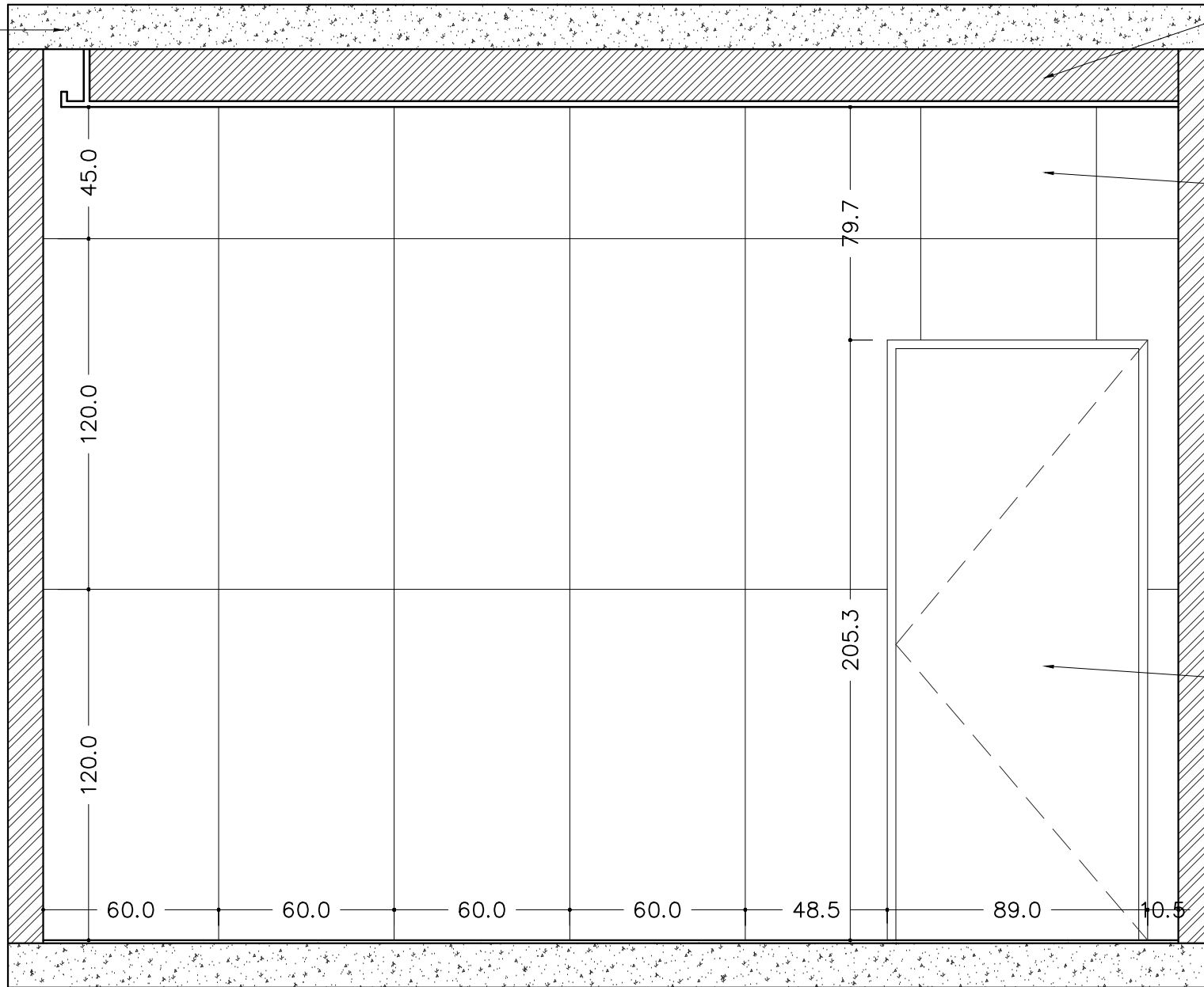
ELEVATION-03
