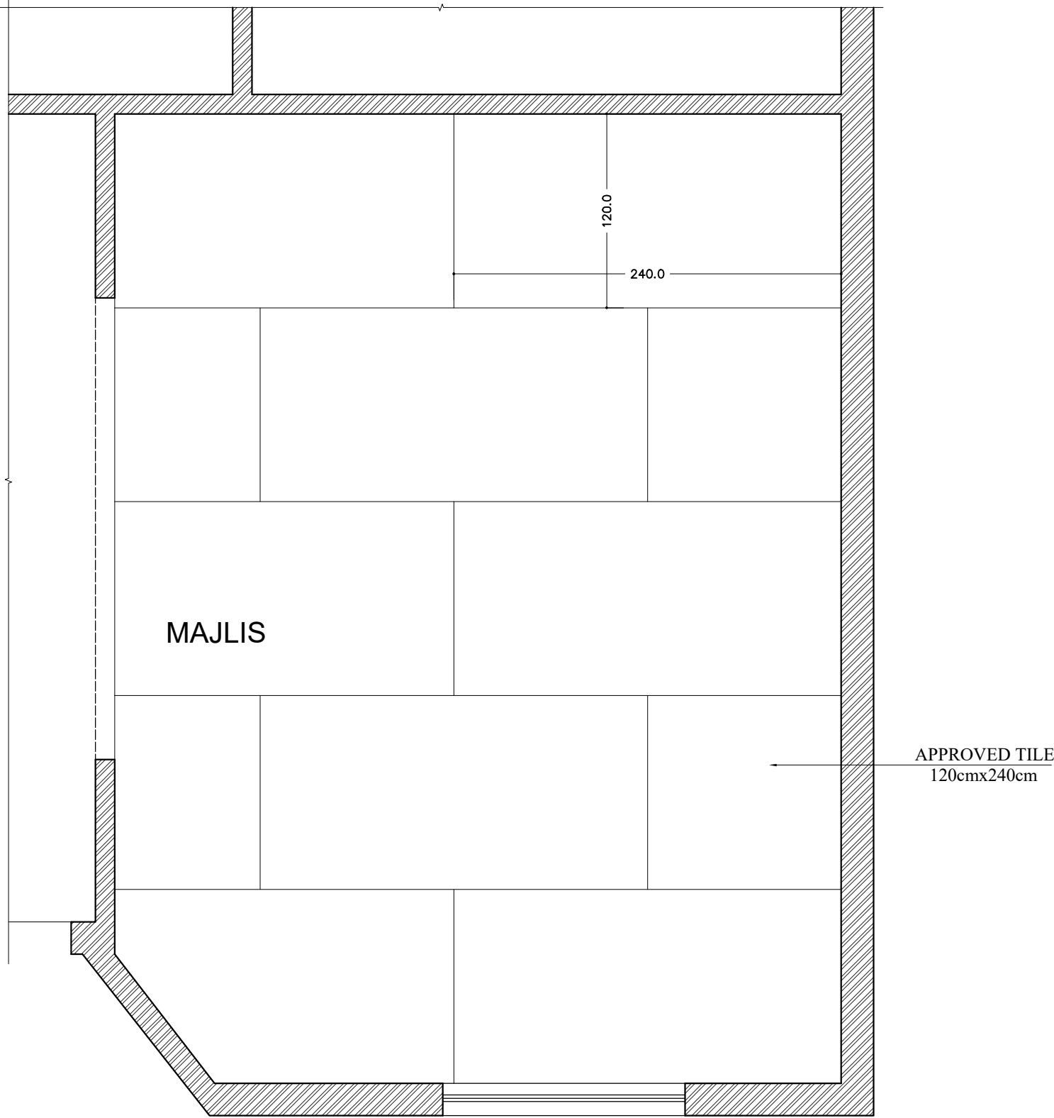
FLOORING LAYOUT PLAN
