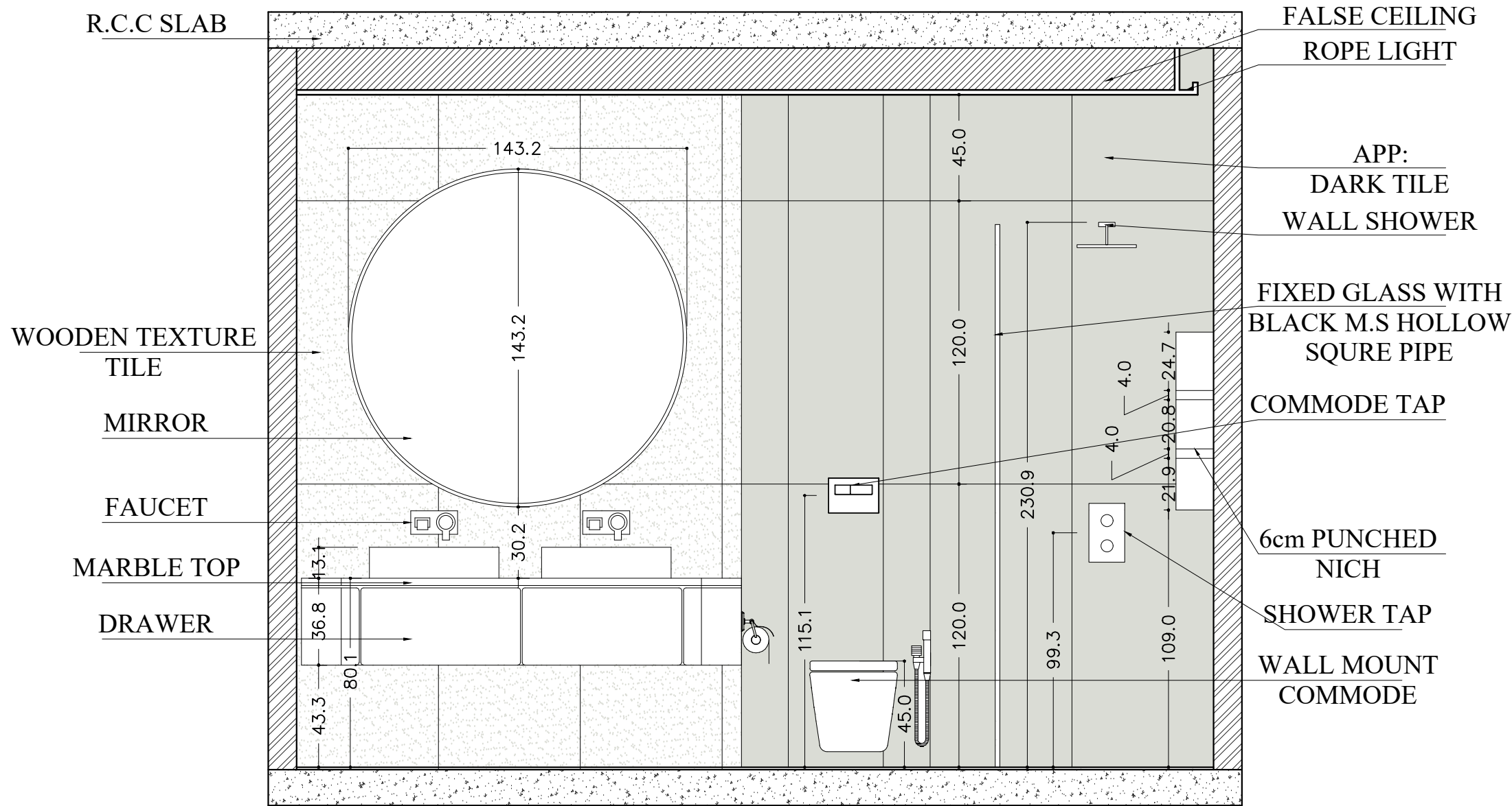
ELEVATION-01
