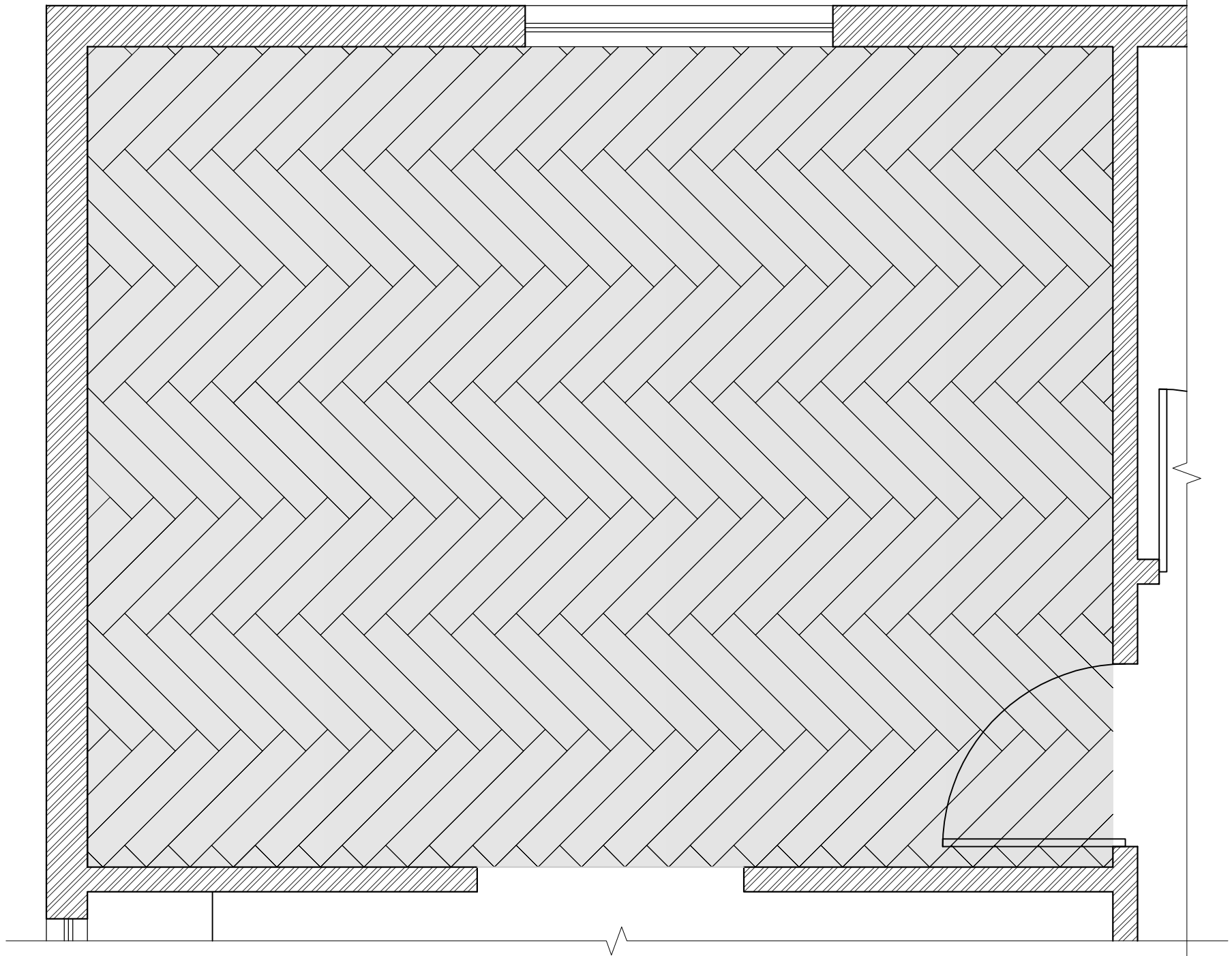
FLOORING LAYOUT PLAN
