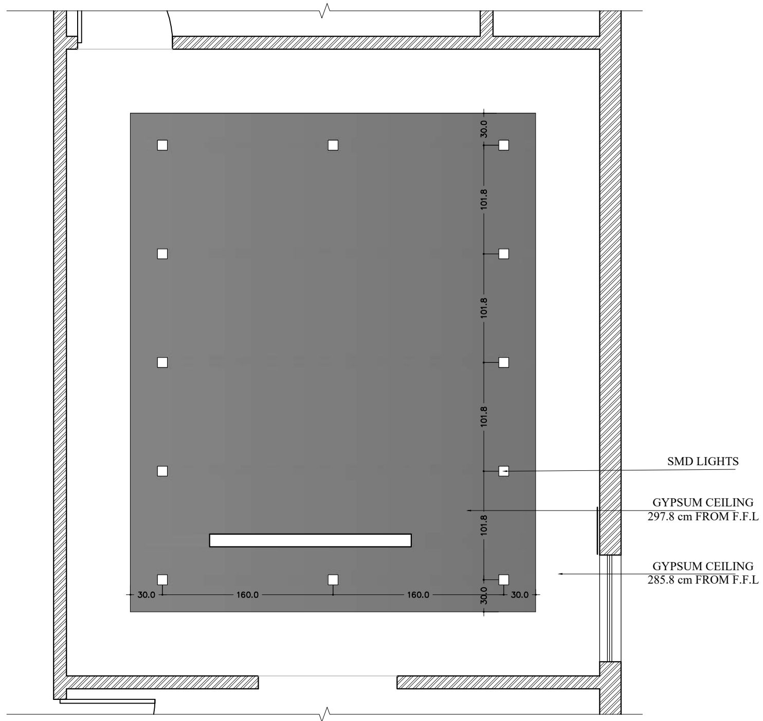
CEILING LIGHT POINT WORKING
