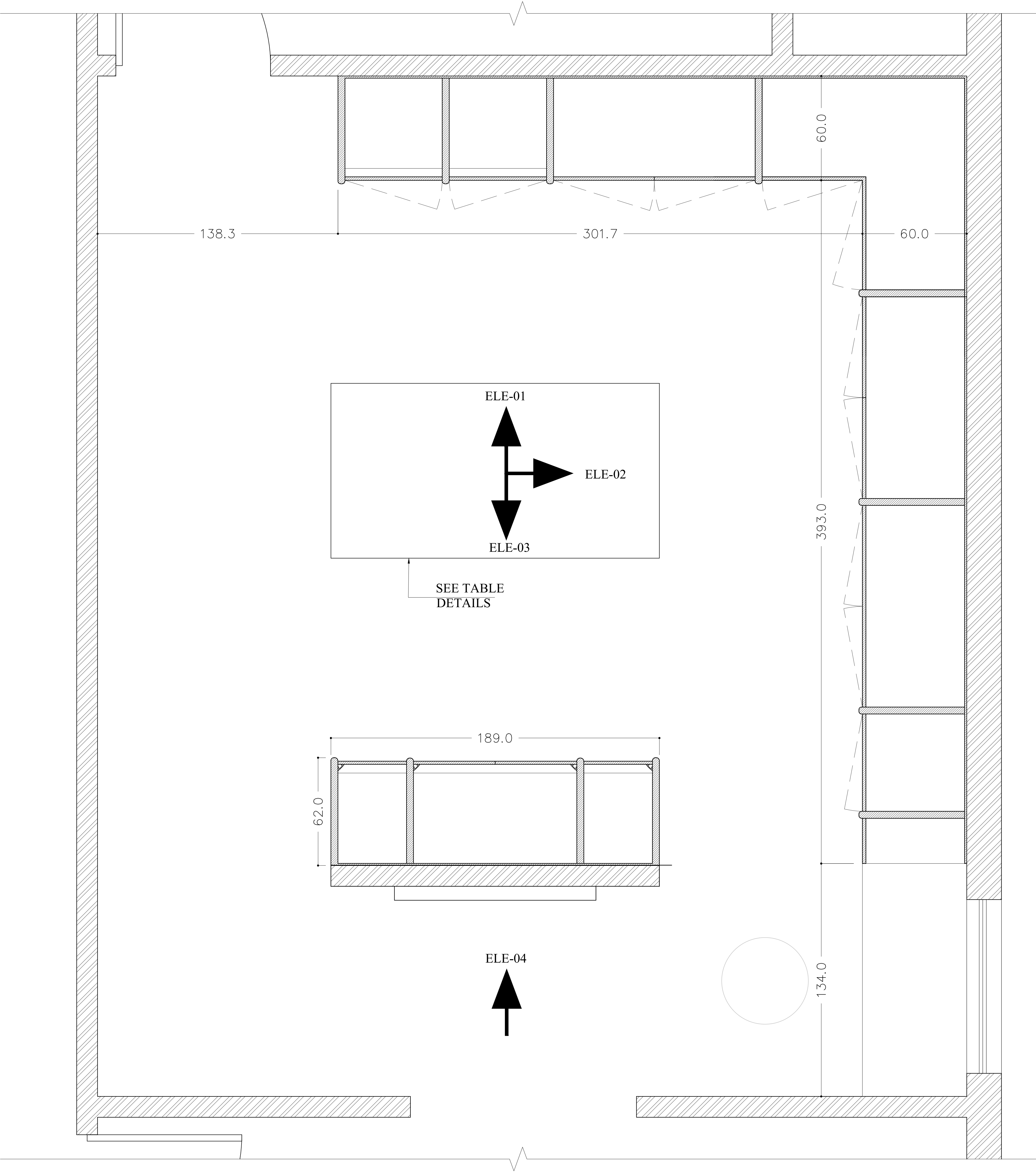
DIMENSION LAYOUT PLAN
