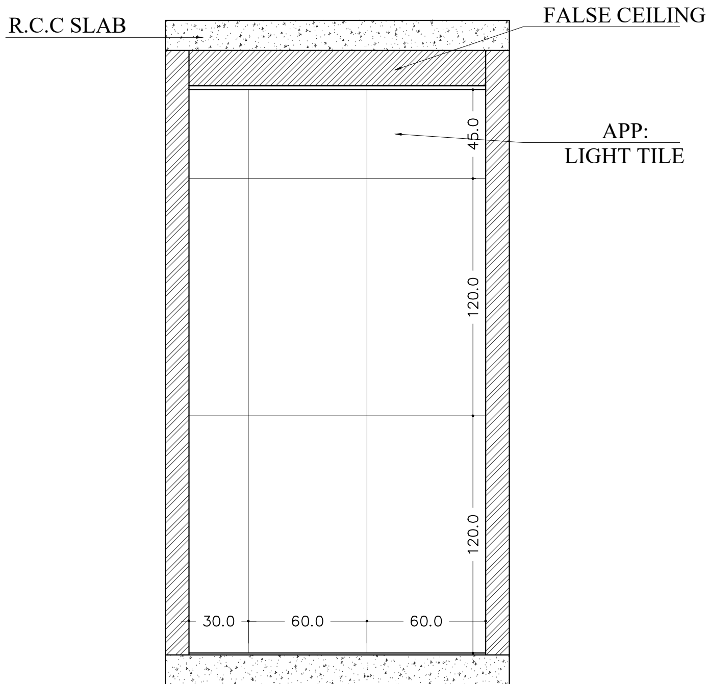
ELEVATION-04
