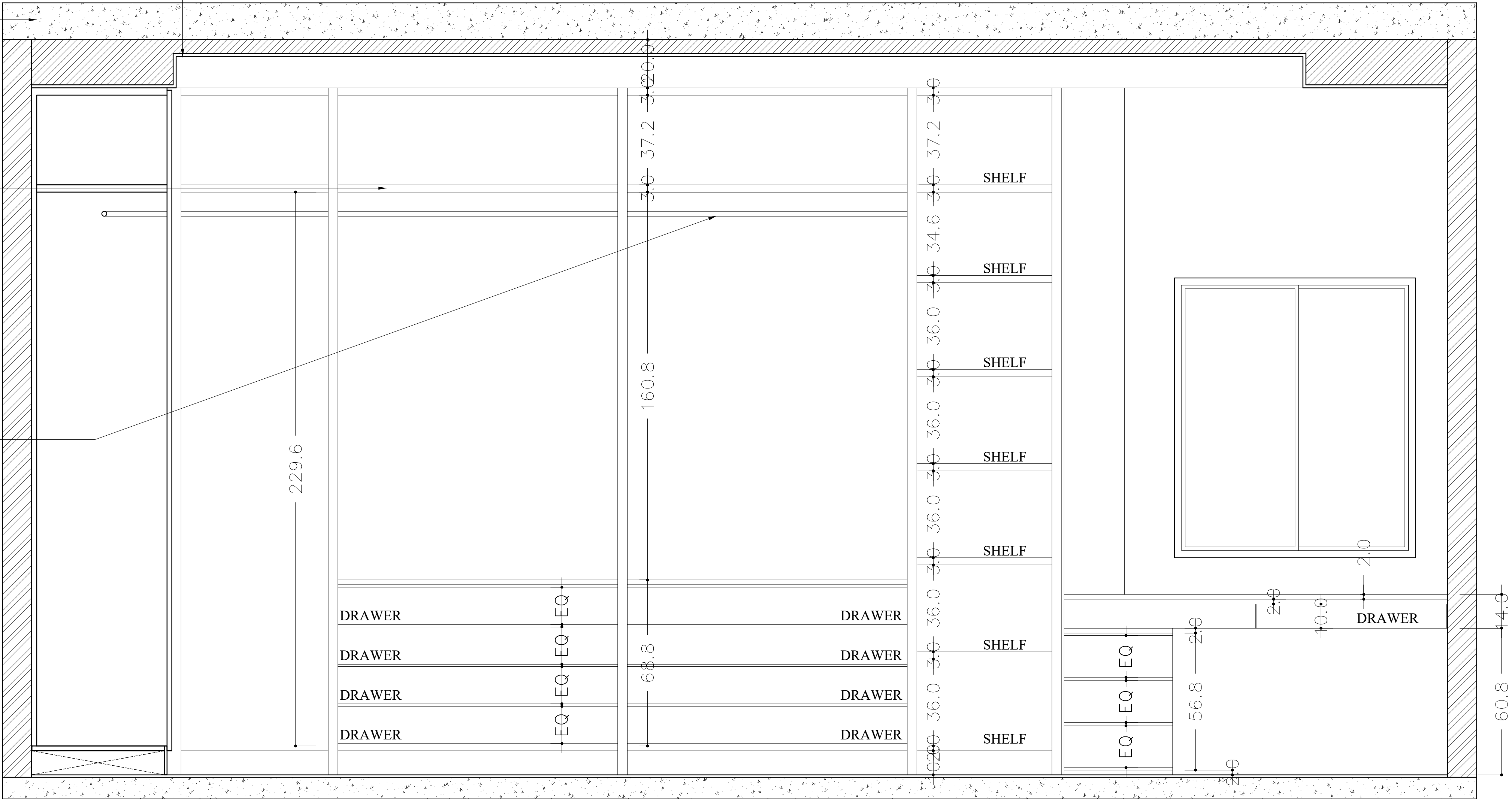
INNER PARTITION WORKING E-02
